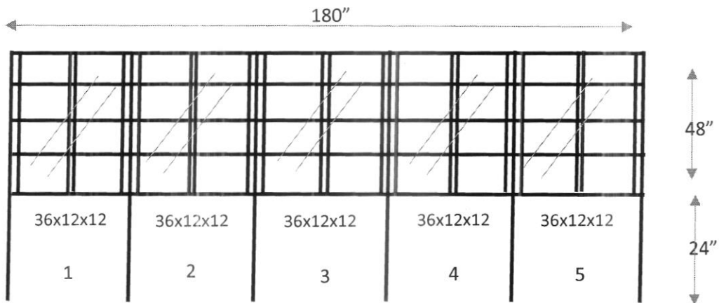
Item 2. Aluminium rack in Dept. Library for keeping books (dimensions in inches)
