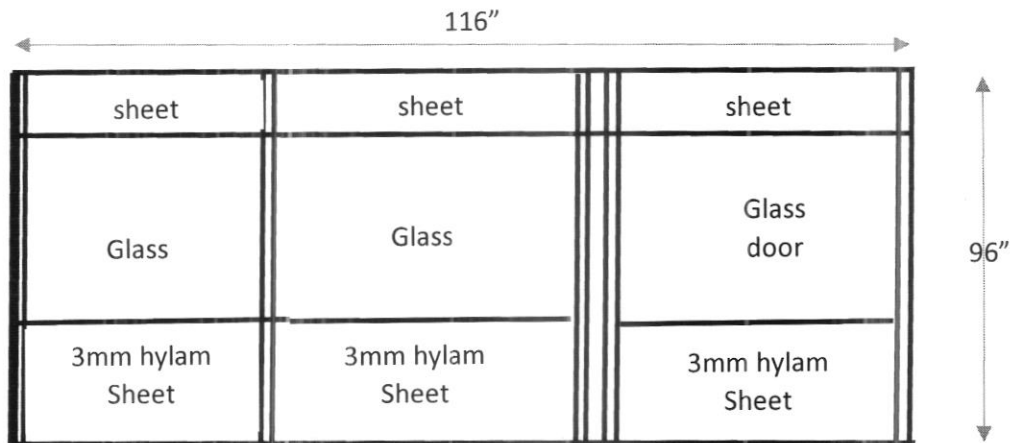
Item 1. Aluminium partition with door (dimensions in inches)
