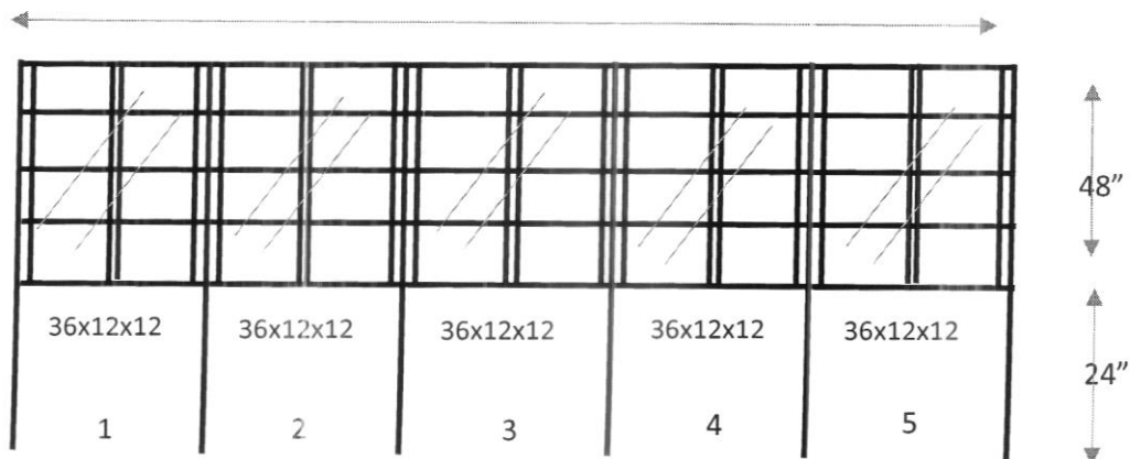
Item 3. Aluminium rack in Room 310 for keeping projects (dimensions in inches)
